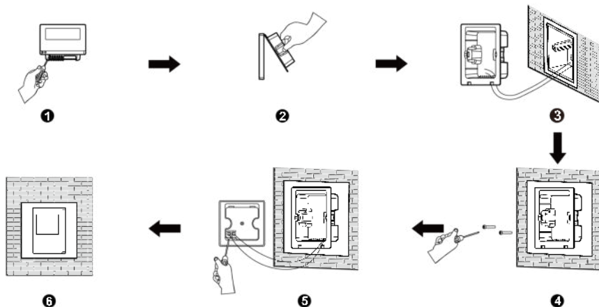
Fig.8-3 Installation of wired controller
