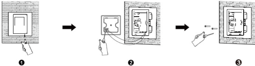
Fig.8-4 Removal of Wired Controller
