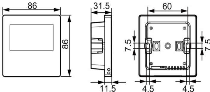
Fig.8-1 Dimensions of Wired Controller
